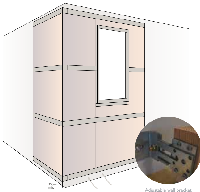
Adjustable wall bracket
